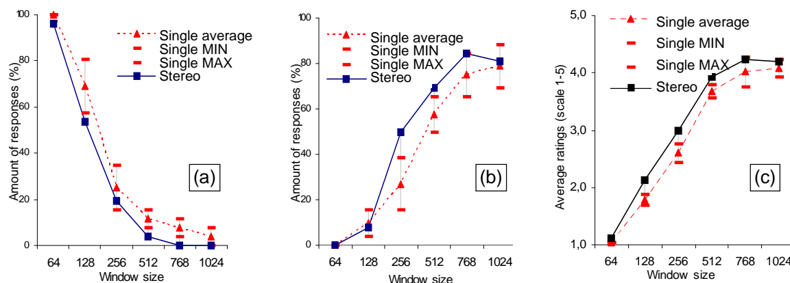
Figure 1. Comparisons between single images (left and right reconstructions) and corresponding stereo images for different window sizes. MIN corresponds to single left or right image that got the least “yes” responses (MAX is most responses). On vertical axis (a) percentage of “yes” responses to: “Does noise disturb substantially?” (b) percentage of “yes” responses to: “Are details completely visible?”, and (c) Evaluated quality using scale 1-5 (1= very poor, 5=very good quality).
