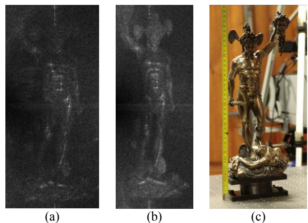
Fig. 17 (a) Amplitude reconstruction of of the object illustrated in (c) using a single beam, (b) and two beams.
