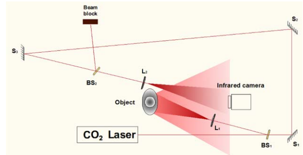
Fig. 10 Off-axis interferometric reflection set-up in reflection mode, S: mirror, L: lens, BS: beam splitter.
