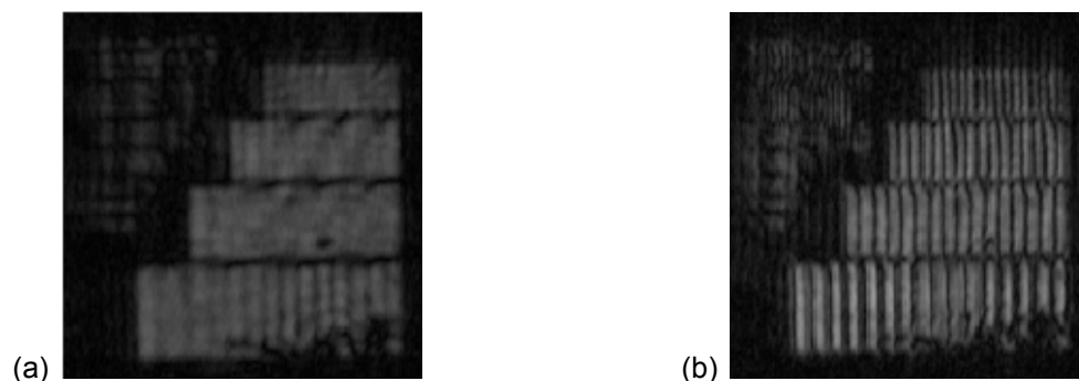
Fig.2. (a) Amplitude reconstruction of the digital hologram acquired when no voltage is applied to the electro-optic grating, (b) super-resolved image obtained through the proposed technique.
